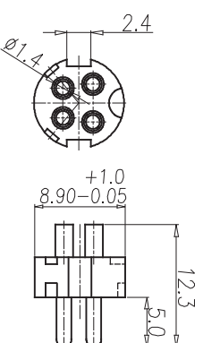
1-1. HOUSING & CONTACT ASSEMBLY
