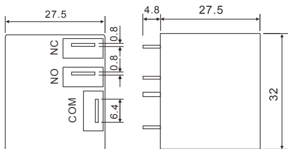
SEALED TYPE
