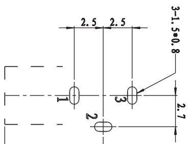
Recommend PCB layout (Jack TOP View)
