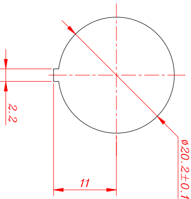
MOUNTING HOLE
