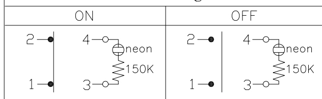
Circuit Diagram
