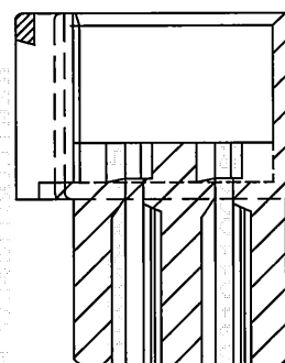
B-B SECTION
