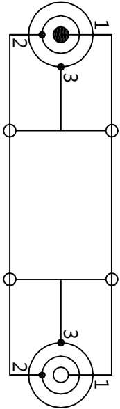
Soldered Drawing: 3.5mm Stereo Plug 3.5mm Stereo Jack
