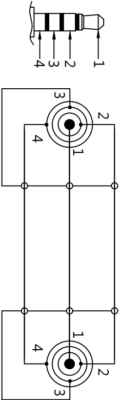
3.5mm 4 Pole Plug 3.5mm 4 Pole Plug
