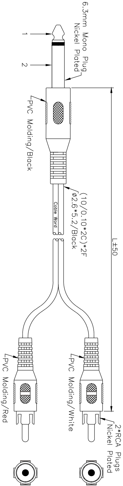
Soldered Drawing: 6.3mm Mono Plug
