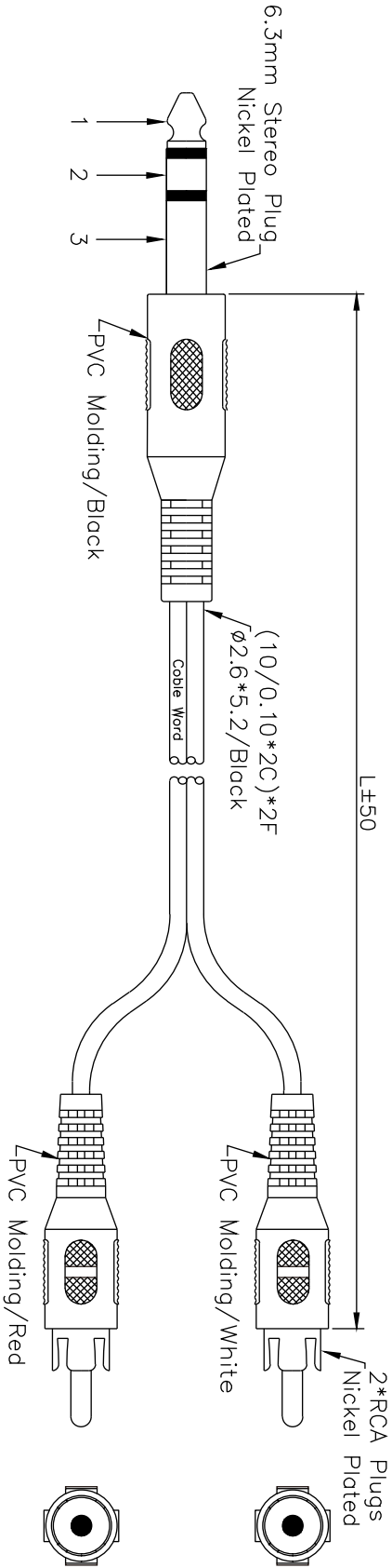
Soldered Drawing: 6.3mm Stereo Plug
