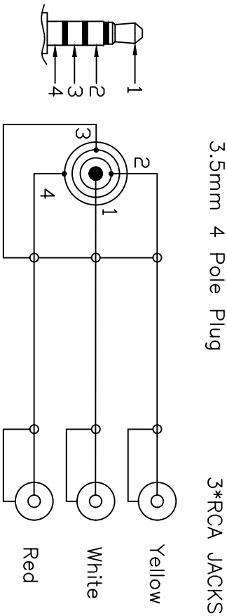
Soldered Drawing:
