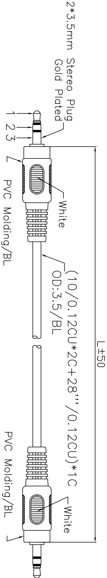
Soldered Drawing:
