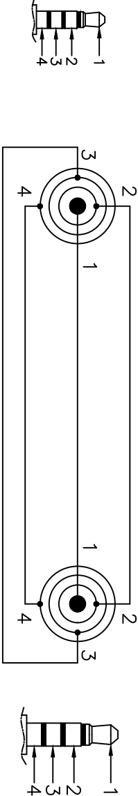
Soldered Drawing: 2.5mm 4 Pole Plug 3.5mm 4 Pole Plug
