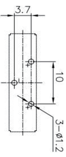
PCB Holes Diagram Top View
