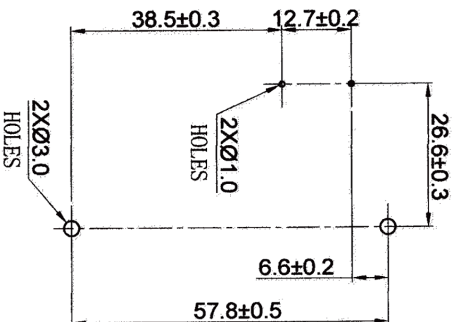
PCB/MOUNTING LAYOUT
