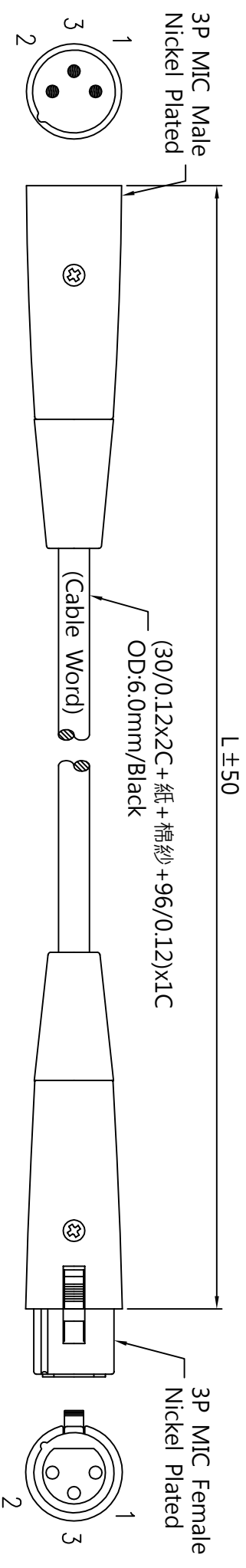
Soldered Drawing:
